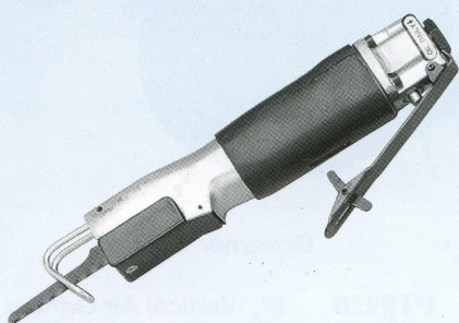
PT313 Air Body Saw 10000 SPM, front exhaust
