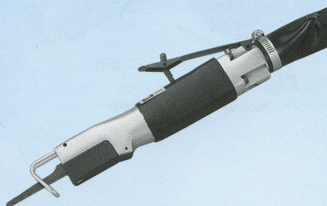
PT313A Air Body Saw 10000 SPM, rear exhaust
